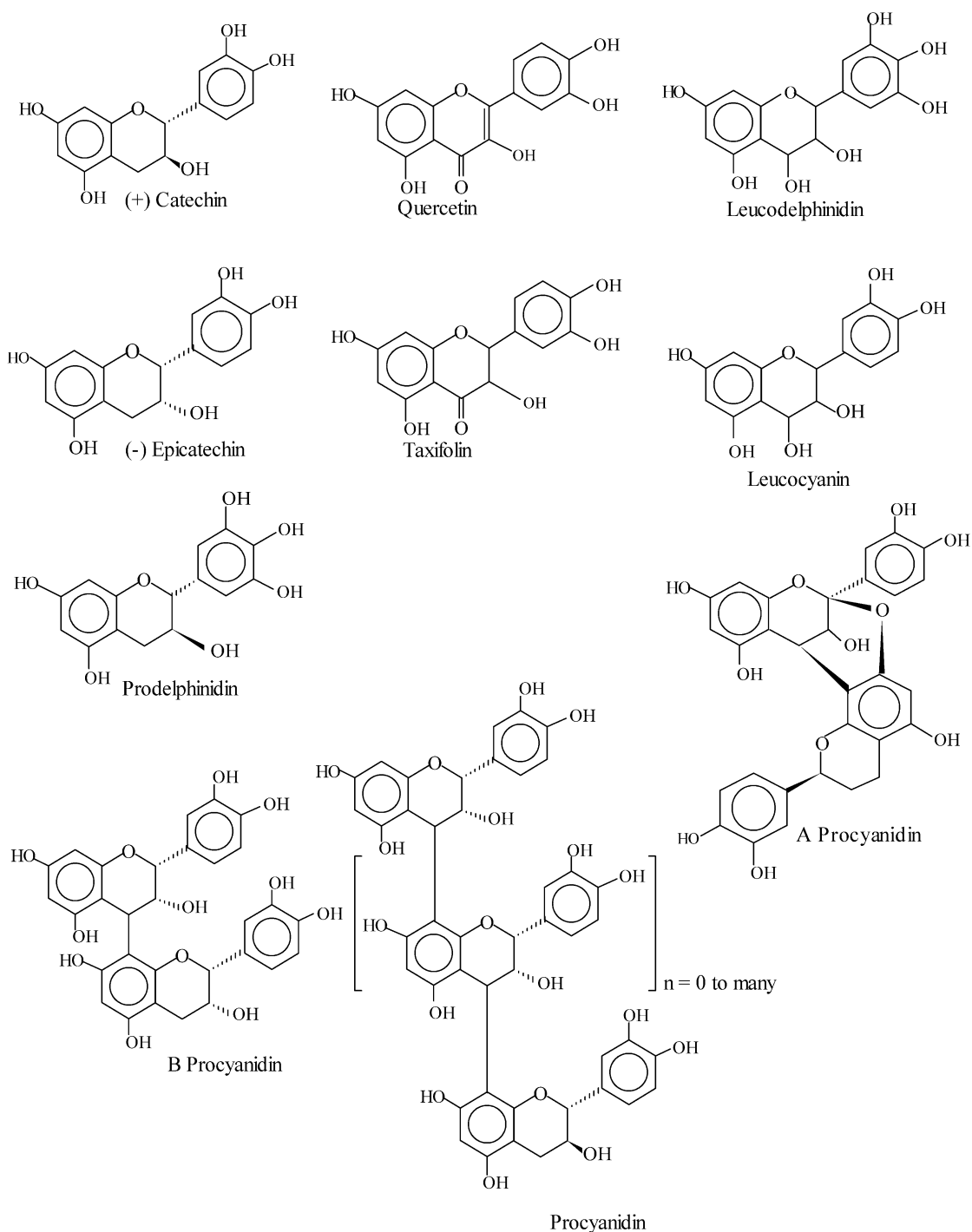
Fig. 2. Flavonoids present in grape skin, grape seed and pine bark extracts.
